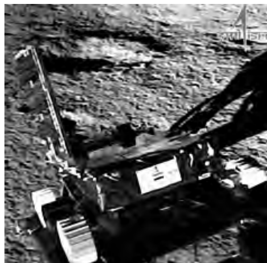
Fig. 6 An image captured by Lander Module [15]
