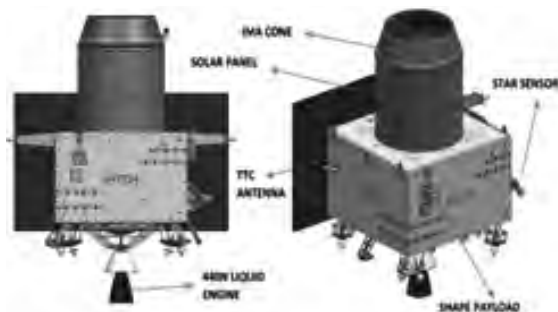
Fig. 1. Transporting the lander-rover payloads to the moon is the primary function of the propulsion module [1]
