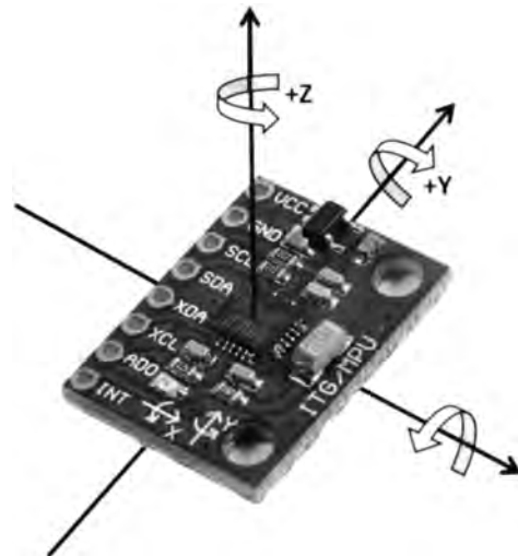
Figure 5. MPU6050 Module
