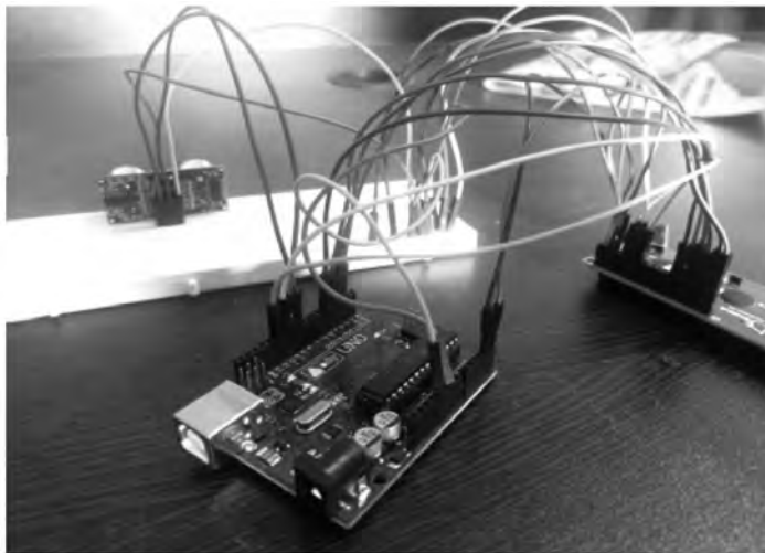
Figure 6. Connections and preliminary hardware prototype of digital measuring tape
