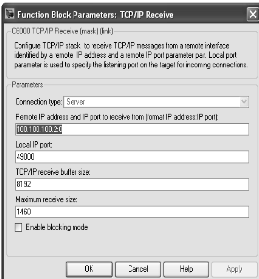
Properties of the simulink TCP/IP receive model
