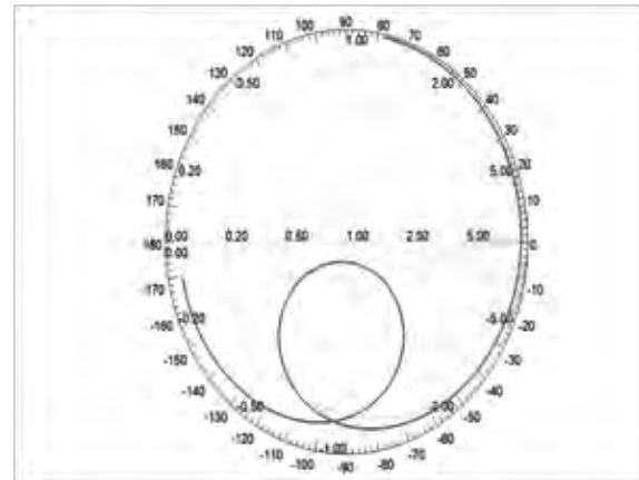
Figure 5: Smith Chart
