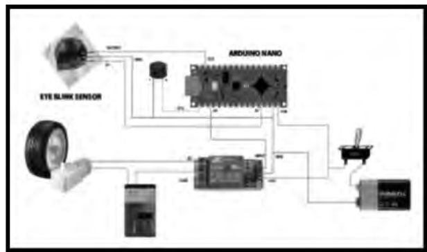
Figure 3: Circuit Diagram
