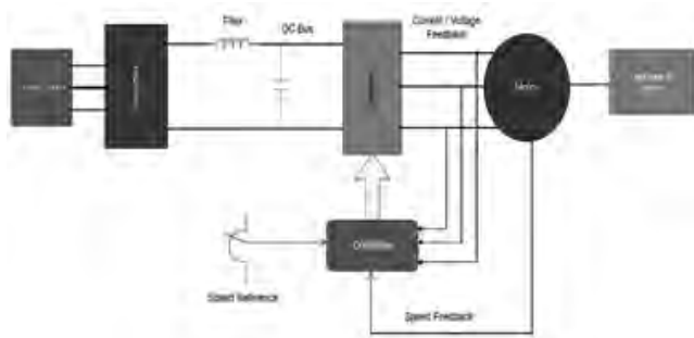
Figure 1. Pictorial representation of variable frequency fed induction motor drive
