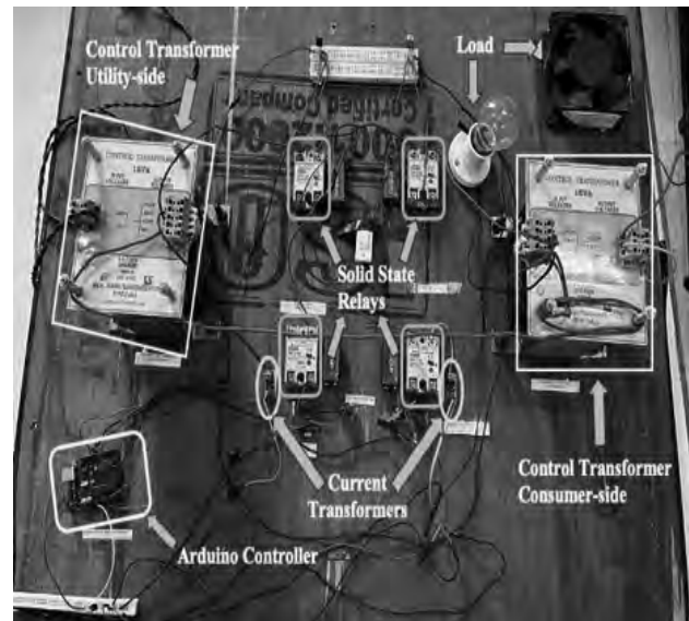
Fig. 5 Experimental set-up of SPDT
