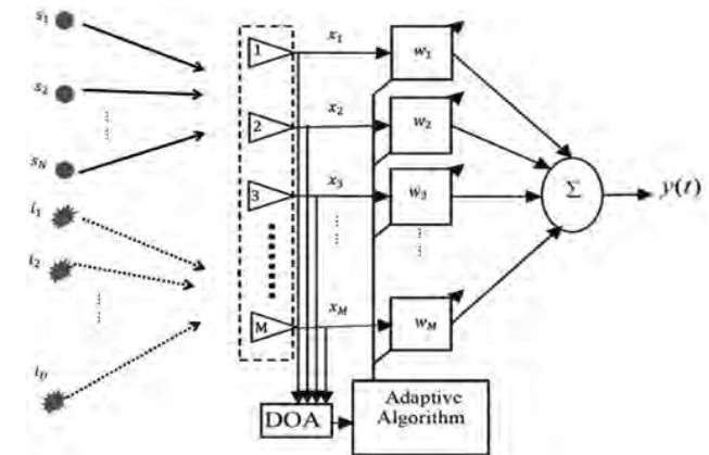
Fig 5: Beam forming antenna [48]
