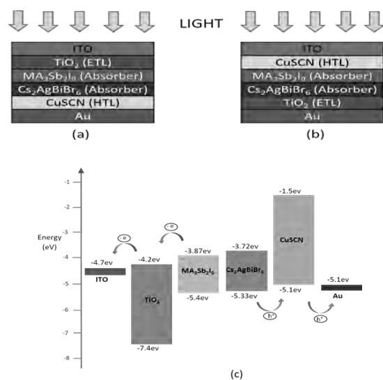
Fig. 1 (a) structural diagram of proposed PSC device (b) structural diagram of inverted PSC device (c) Energy band diagram and the carrier transport mechanism in \text{MA}_3\text{Sb}_2\text{I}_9 and \text{Cs}_2\text{AgBiBr}_6 based PSC device.
