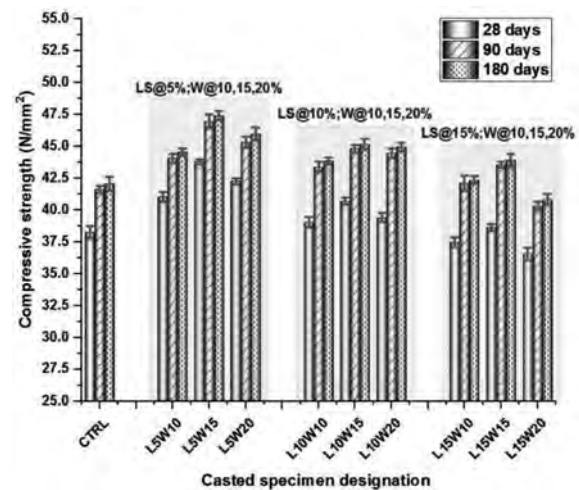
Figure 4. Compressive strength behavior of WM-LS concrete mixes
