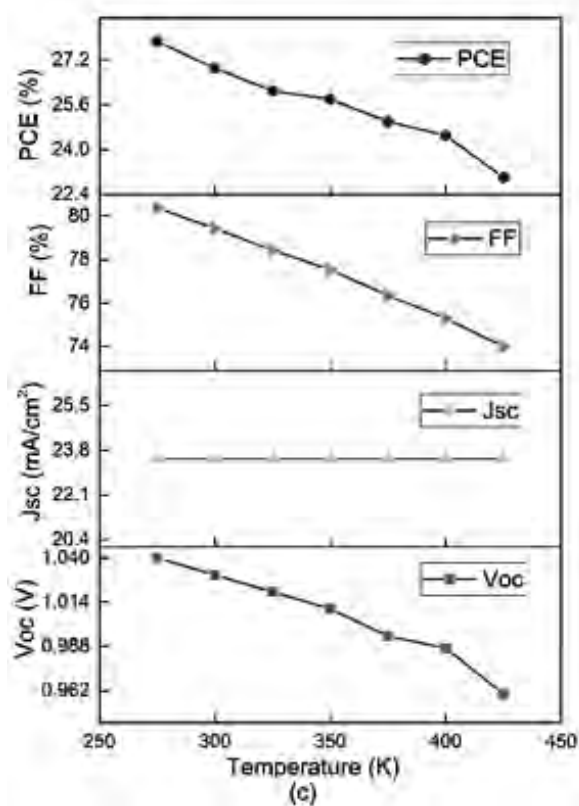
Fig. 4. Shows the variation of Solar cell parameters with respect to Temperature, Shunt Resistance and Series Resistance. (a) Series Resistance variation effect on FF, J_{sc} , V_{oc} and PCE. (b) Shunt Resistance variation effect on FF, J_{sc} , V_{oc} and PCE (c) Temperature variation effect on FF, J_{sc} , V_{oc} and PCE.
