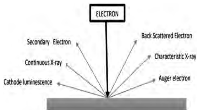
Figure 2. Working Principle of SEM
