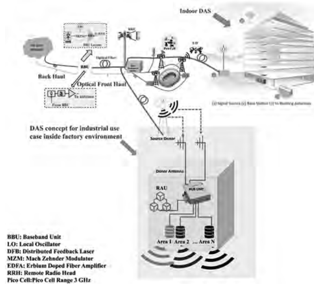
Fig 3: Small cell antennas [46]
