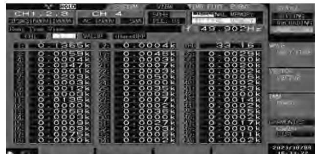
Figure 5: VFD input current harmonic measurement at full load
