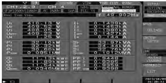
Figure 2: Input parameters of VVVF fed induction motor drives
