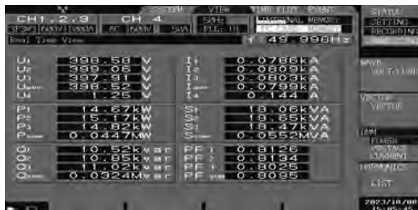
Figure 13: Output waveforms of VVVF fed induction motor drives dynamic performance at 50 percent load
