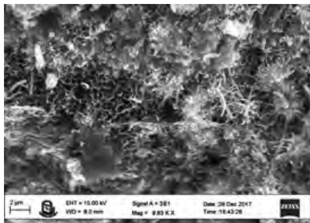
Figure 5. Evenly Distribution of Hydrated Products with crystals in Concrete Structure
