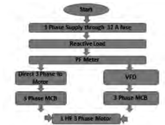
Fig. 3 Flowchart of system
