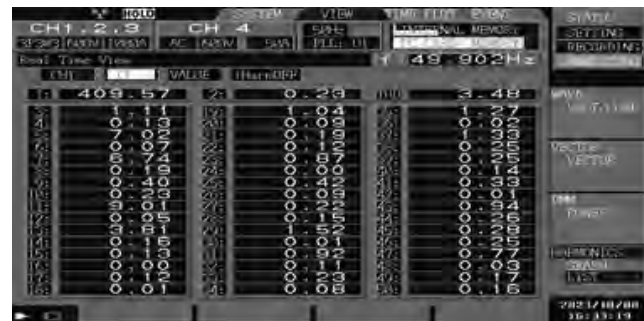
Figure 4: VFD input voltage harmonic measurement at full load
