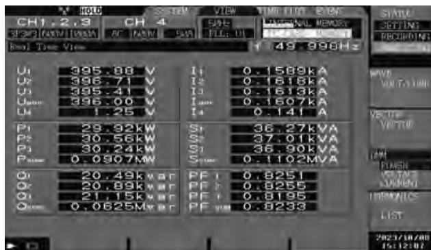
Figure 8: Output parameters of VVVF fed induction motor drives dynamic performance at full load
