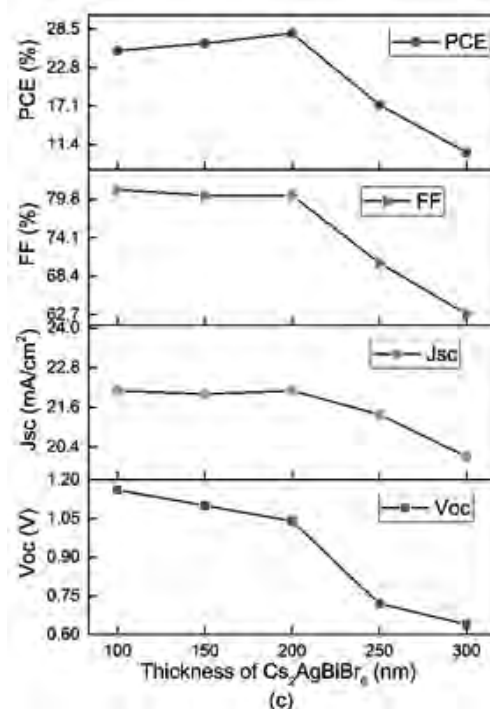
Fig. 3. Shows the solar cell parameters variation with respect to thickness and defect density of PAL. (a) Defect density variation of \text{MA}_3\text{Sb}_2\text{I}_9 and \text{Cs}_2\text{AgBiBr}_6 effect on FF, J_{sc} , V_{oc} and PCE. (b) Thickness variation of \text{MA}_3\text{Sb}_2\text{I}_9 effect on FF, J_{sc} , V_{oc} and PCE (c) Thickness variation of \text{Cs}_2\text{AgBiBr}_6 effect on FF, J_{sc} , V_{oc} and PCE.
