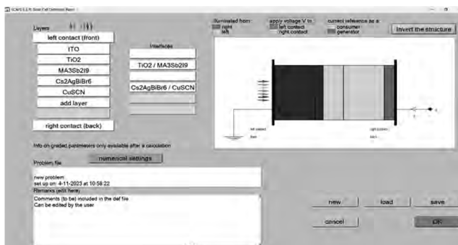
Fig. 2 Picture of SCAPS 3.3.10 Definition Panel containing the proposed structure.
