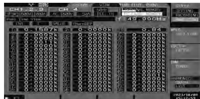
Figure 6: VFD output voltage harmonic measurement at full load
