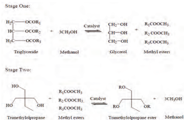
Fig. 1. Production of Palm based WCO TMP Esters
