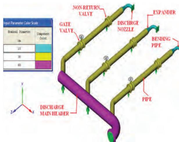
Fig. 4 Geometric plot of discharge pipe
