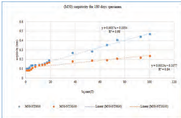
Graph 10: Sorptivity for 180 days specimen (M50)
