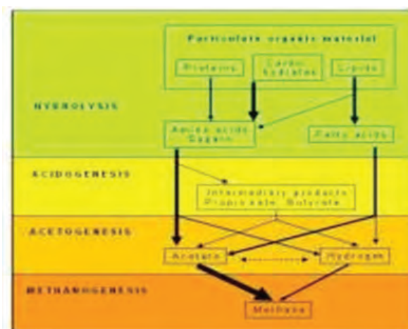
Fig. 1. Flow chart for biodegradation
