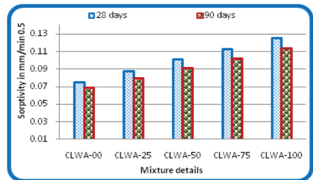
Fig. 7 Sorptivity of Various mixtures
