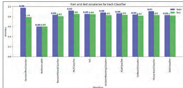
Fig. 13: All Classifiers Train-Test Accuracy Bar Chart-using Word2vec for Skip-gram
