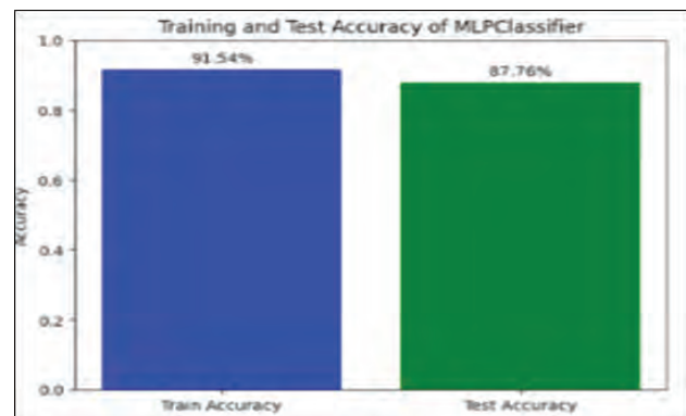
Fig. 22 MLP after hyperparameter tune
