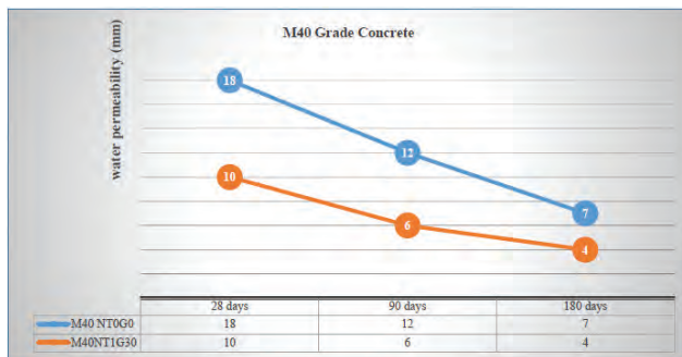
Graph 3: Water Permiability- M40
