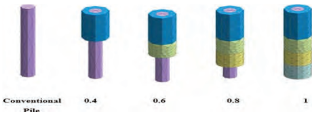
Fig 3: Geometry Modeling of a Pile Encased with Sand Cushion
