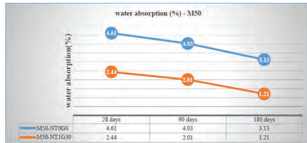
Graph 2: water absorption (%) for M50 grade concrete.
