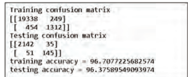
Fig. 10 Accuracy and confusion matrix of SVM
