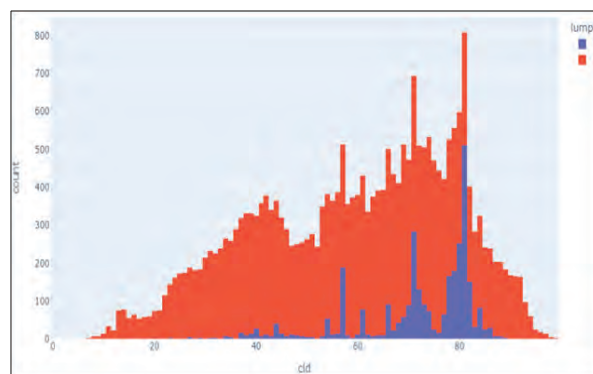
Fig. 4 Analysis of Monthly Cloud Cover
