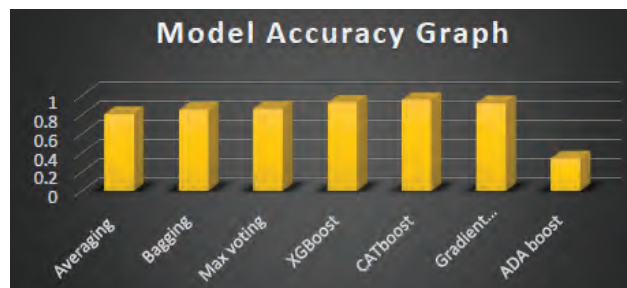
Fig. 4 : Accuracy Graph
