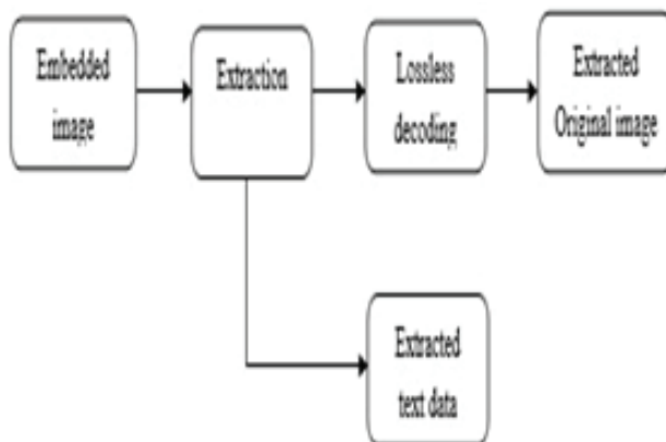
Fig.3. RDH Extraction
