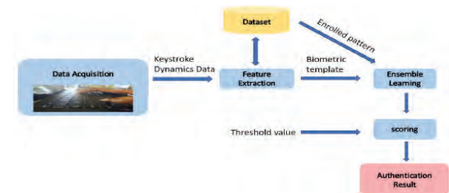
Fig. 3: Methodology
