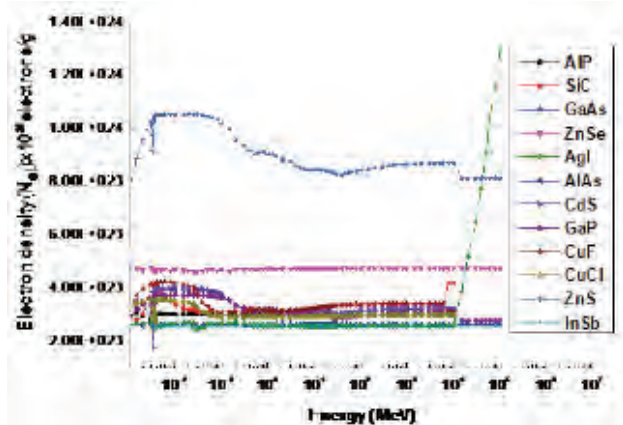
Fig. 7. Variation of the N_{el} as function of energy for coherent process.
