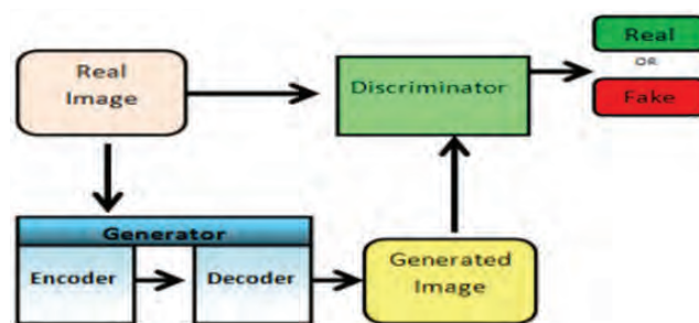
Fig. 1 Architecture of GAN image anomaly detection
