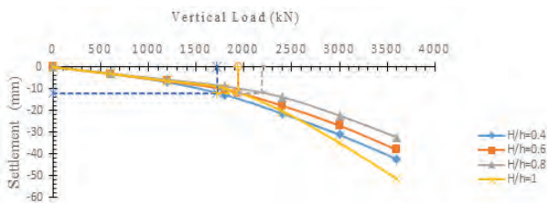
Fig. 11: Load-Settlement curve for h_p = 12 m & Dr = 1.2 ( d_p = 600 mm, D = 720 mm)
