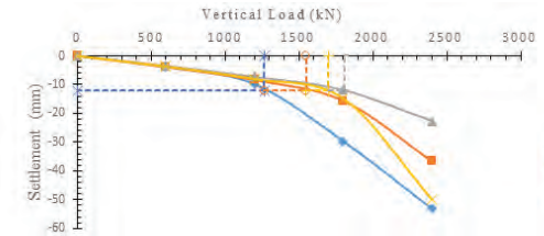
Fig. 9: Load-Settlement curve for h_p = 9 m & Dr = 1.8 ( d_p = 600 mm, D = 1080 mm)
