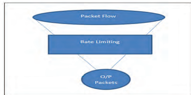
Fig. 3. Rate limiting
