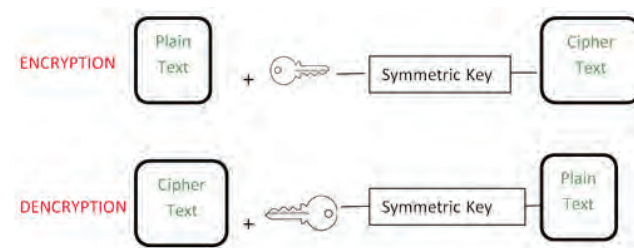
Fig. 1. Cryptography process
