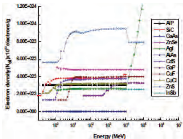
Fig. 11. Variation of the N_{\text{el}} as function of energy for pair nuclear process.
