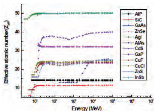
Fig. 12. Variation of the Z_{\text{eff}} as function of energy for pair electron process.
