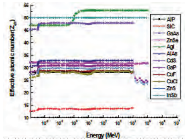
Fig. 8. Variation of the Z_{eff} as function of energy for incoherent process
