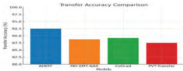
Fig. 6: Transfer Accuracy Comparison across Models
