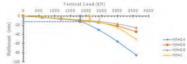
Fig. 14: Load-Settlement curve for h_p = 12 m & Dr = 1.8 ( d_p = 600 mm, D = 1080 mm)
