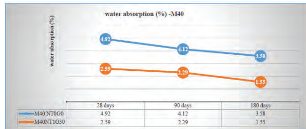
Graph 1: water absorption for M40 grade concrete
