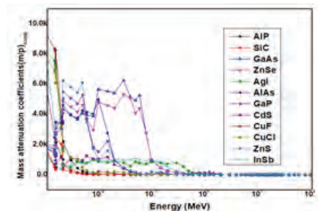
Fig 1. Variation of mass attenuation coefficient of crystalline materials in the energy region 1keV-100 GeV for photon interaction (with coherent).
