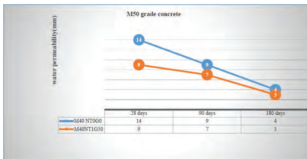
Graph 4: Water Permiability- M50
