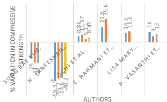
Fig. 6. Percentage Variations in tested properties
