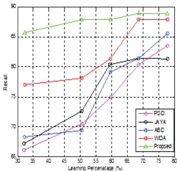
Fig. 7: Recall
