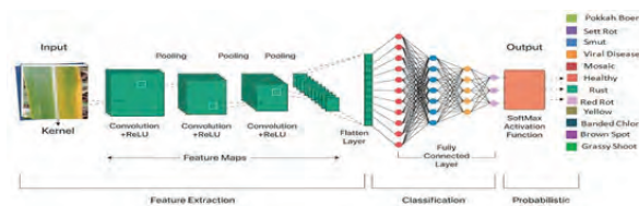
Fig. 3: Overview structure of the Proposed Model (SugarNet)
