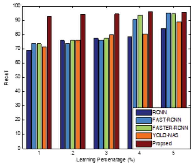
Fig. 11: Recall
