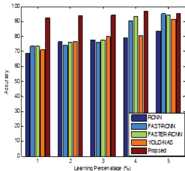
Fig. 8: Accuracy
