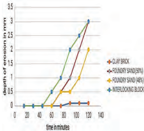
Fig 9: Plot of Depth of erosion v/s Time for various building materials
