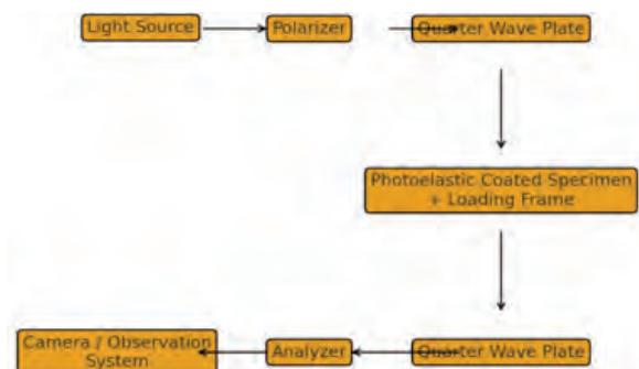
Fig. 5.2: Experimental setup
