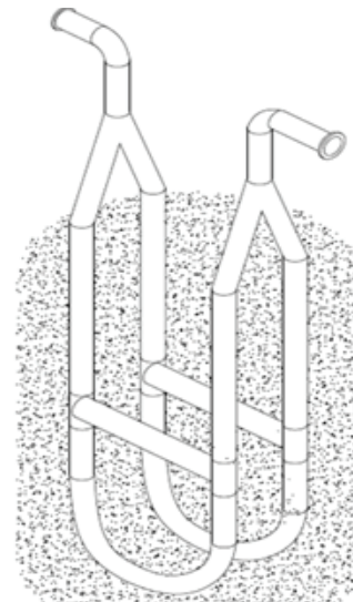
Fig. 6: Schematic diagram of Vertical BTHE
