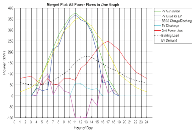
Fig. 10. PV generation, PV power used for EV, BESS discharging and charging, Grid power used, EV demand
