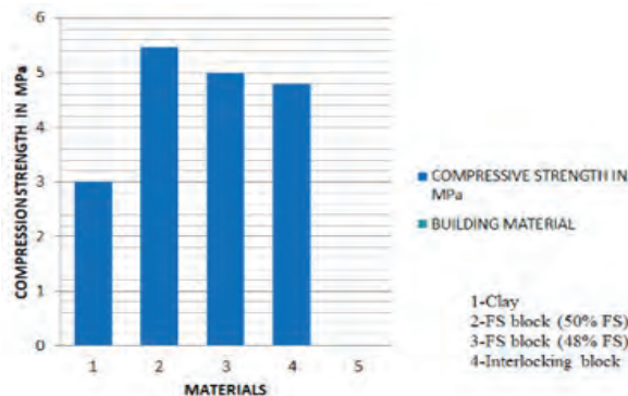
Fig. 8: Plot of various building Materials v/s compressive strength test results
