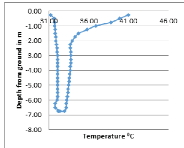
Fig. 10: Temperature profile of ambient air travel in Vertical BTHE during Simulation
