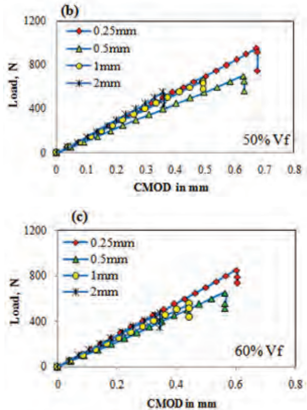
Fig. 3. Load v/s CMOD curves of CPE Composite specimens for different Particle Sizes in (a) 40% Vf (b) 50% Vf and (c) 60% Vf
