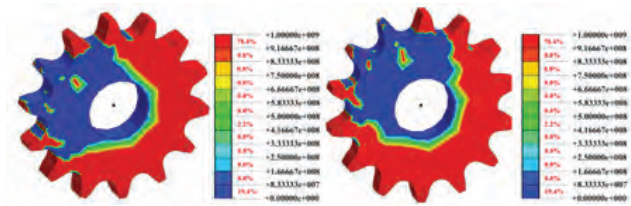
Fig. 4.7: Investigation of stresses in condition-3 by ANSYS
