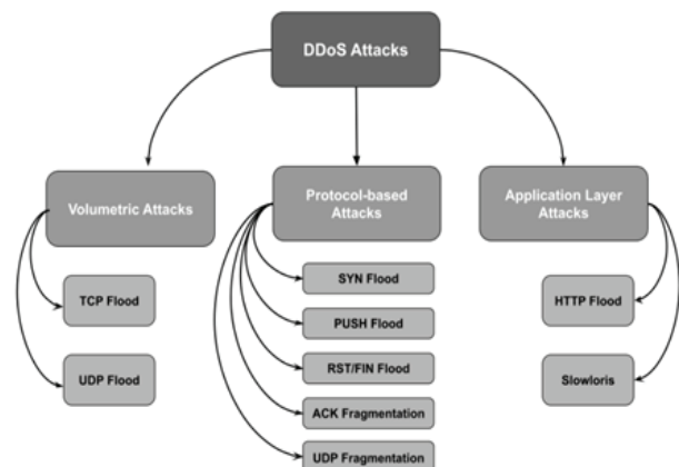
Fig. 2: DDoS Attacks Classification
