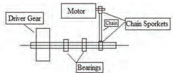
Fig. 5.1: Schematic diagram of experimental setup
