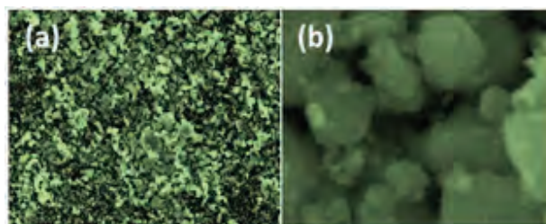
Fig. 4 (a, b) FE-SEM images of the SnO 2 sample
