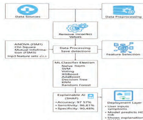
Fig. 1: System Architecture Diagram
