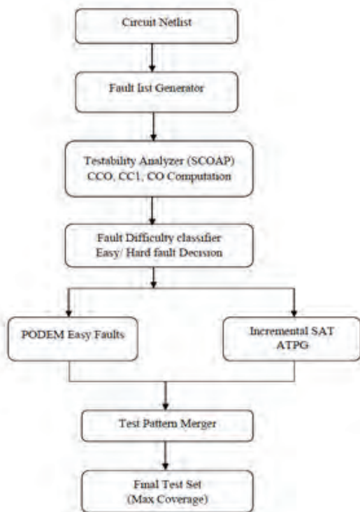
Fig. 1 : Architecture of proposed work
