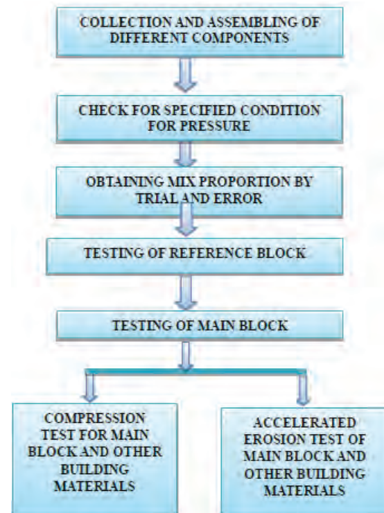
Fig. 5: Flow chart depicting different stages of tests
