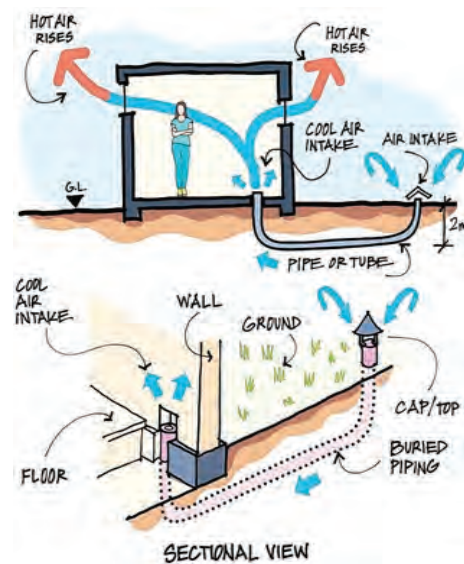
Fig. 3: Sectional View of Horizontal BTHE
