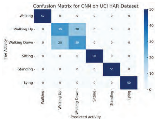
Fig. 4: Confusion Matrix for CNN and UCI Dataset
