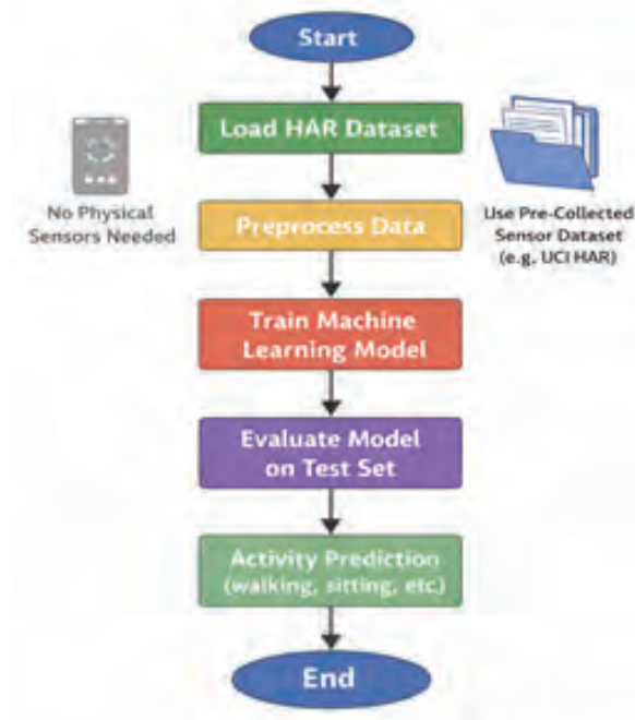
Fig. 1: Workflow for a Human Activity Recognition (HAR) system
