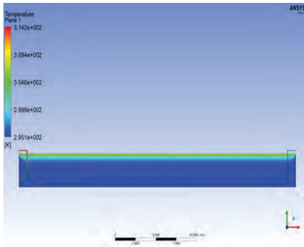
Fig. 2: CFD Modelling of Buried Tube Air Conditioning System
