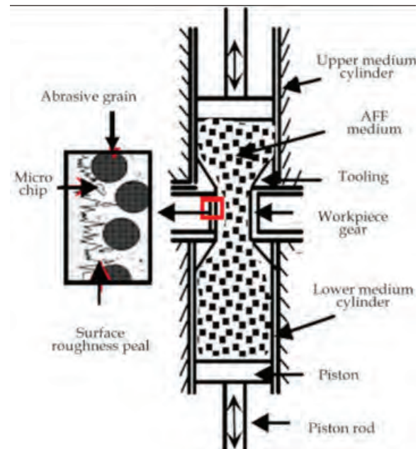
Fig. 1: Experiment set up schematic diagram
