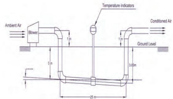
Fig. 3.1: Schematic diagram of Horizontal BTHE
