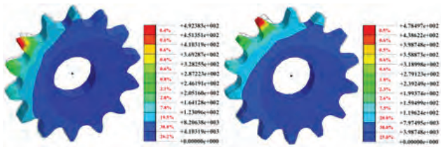
Fig. 4.6: Stress analysis for condition-2 by ANSYS
