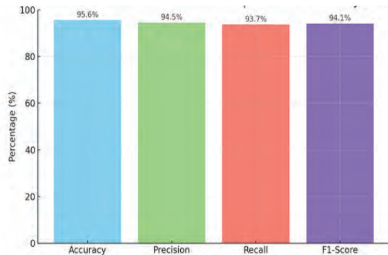
Fig. 8: Evaluating performance include accuracy, precision, recall, F1-score
