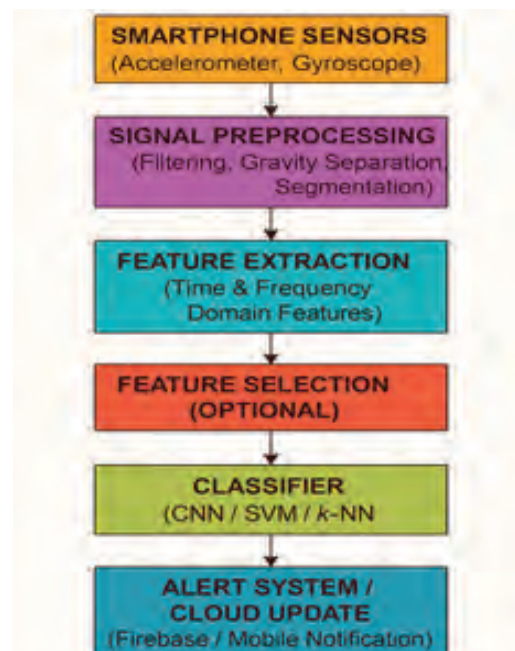
Fig. 2: Flow Diagram for Smartphone Based Activity Recognition
