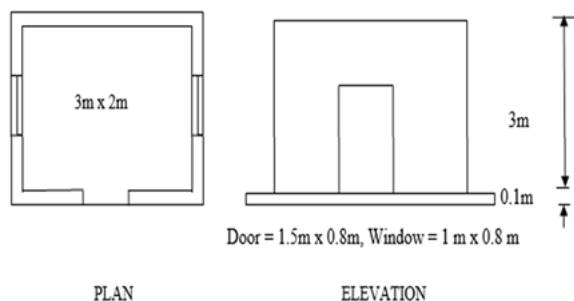
Fig. 1: Plan and Elevation of the Model
