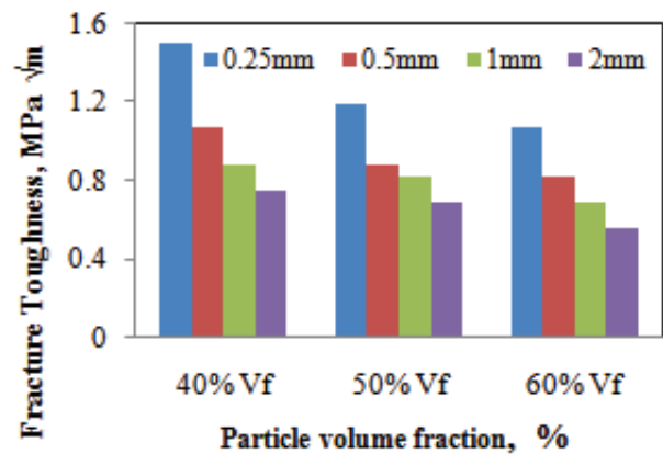
Fig.6. Fracture Toughness of CPE Composite specimens
