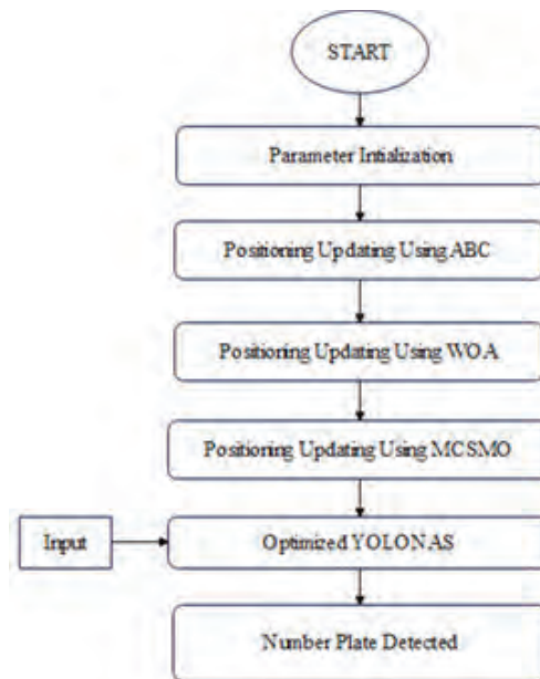
Fig. 2: Flow Chart of Proposed Model
