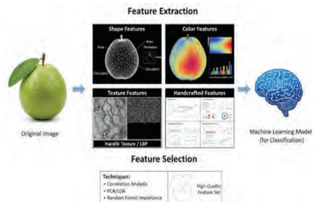
Fig. 6: Feature Extraction and Selection for Guava fruit
