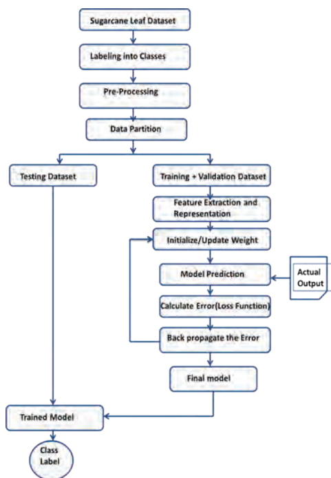
Fig. 2: Schematic Flowchart of Proposed Model (SugarNet)
