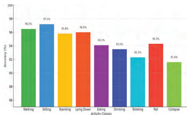
Fig. 5: Activity Recognition Accuracy on Elderly AR Dataset
