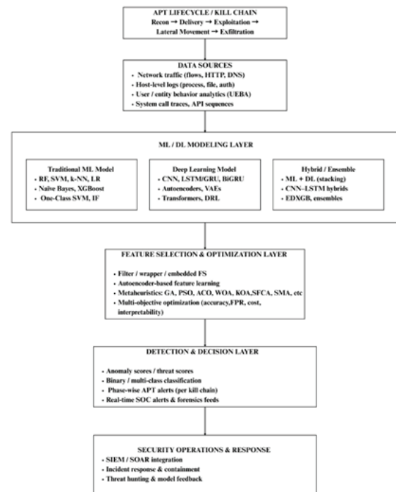
Fig. 1 : Unified Taxonomy of ML, DL, and Optimization-Based APT Detection Frameworks
