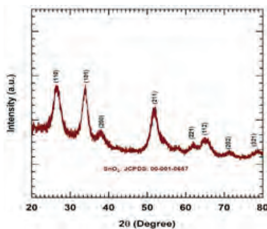
Fig. 3: XRD pattern of SnO 2 sample
