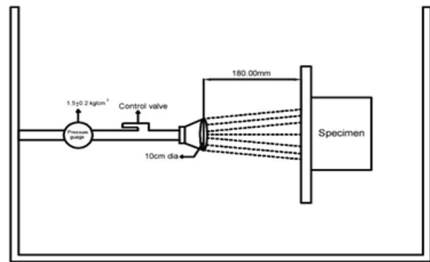
Fig. 6: Schematic view of accelerated erosion test apparatus
