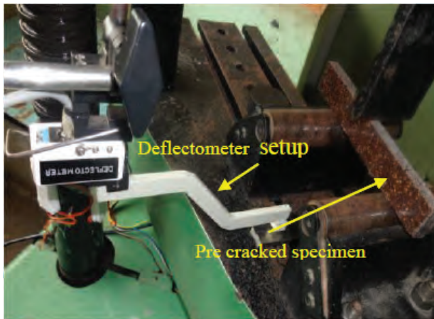
Fig.2. Configuration of Fracture Toughness Test Setup
