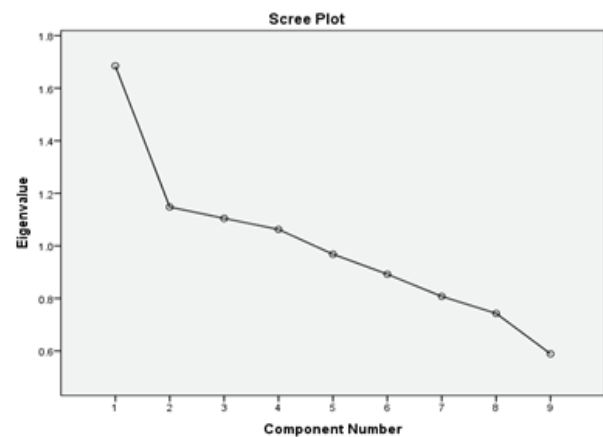
Fig. 1: Scree Plot
