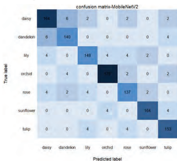
Fig. 3: Confusion Matrix
