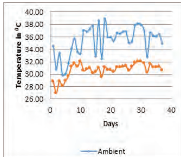
Fig. 12: Temperature profiles of ambient or inlet air and outlet air from Vertical BTHE
