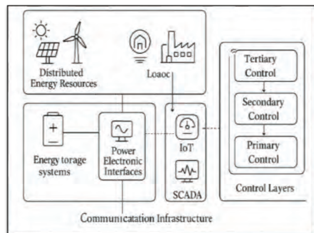
Fig. 1: Architecture of Smart Microgrid
