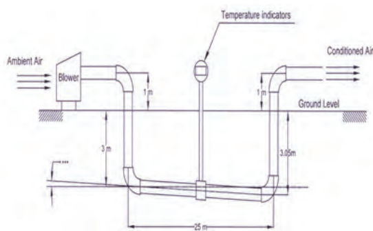
Fig. 5. Horizontal Buried tube heat exchanger
