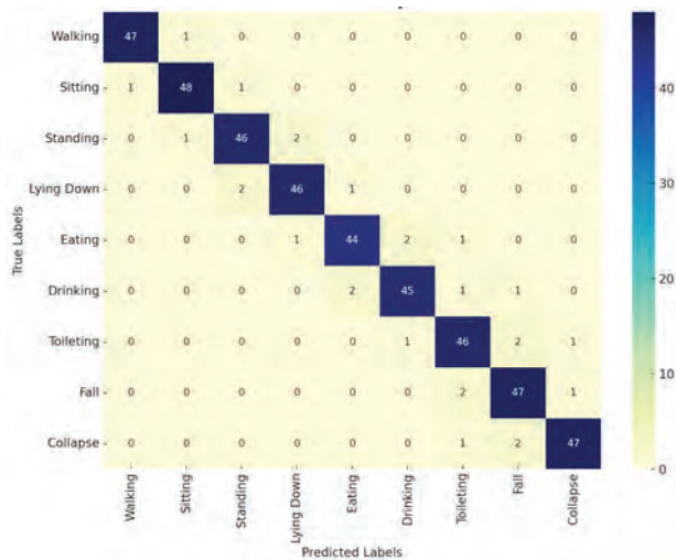
Fig. 6: Confusion Matrix Elderly AR Dataset
