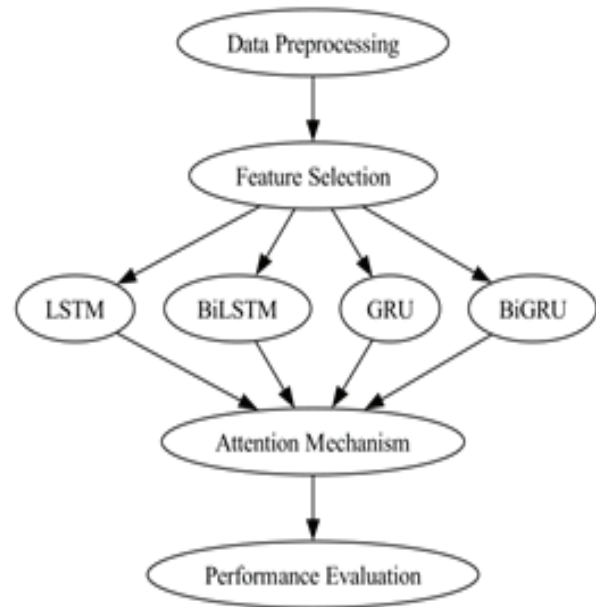
Fig. 1 proposed framework for CCI forecasting.
