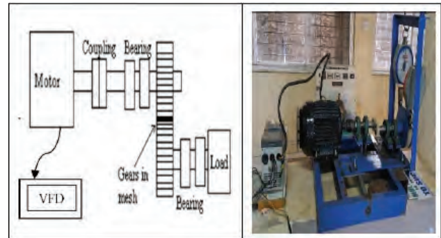
Fig. 1: Gear Test Dynamic Test Set-up
