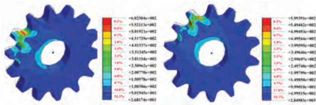
Fig. 4.5: Stress analysis for condition-1 by ANSYS
