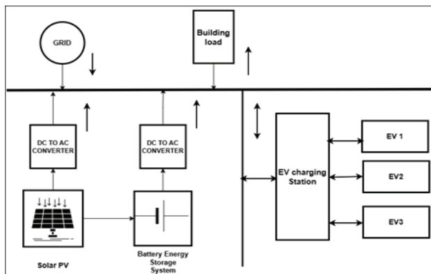
Fig. 1: Solar-PV Grid assisted EV charging station
