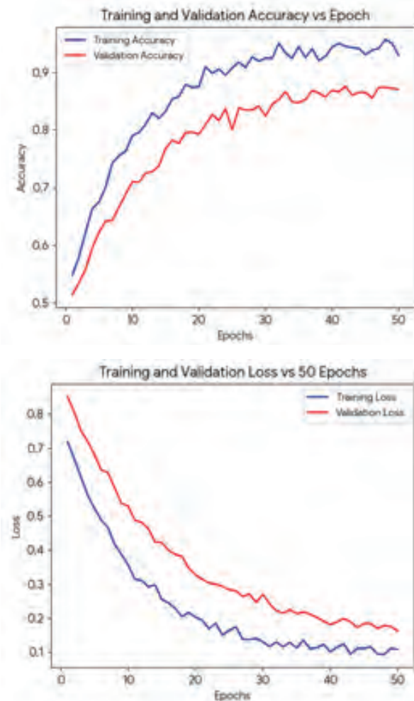
Fig. 2: Training and Validation Accuracy and Loss Plot
