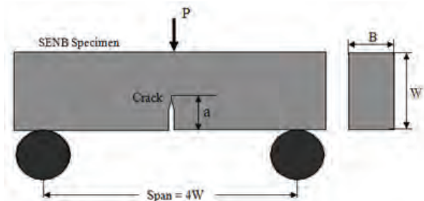
Fig.1. SENB test Sample
