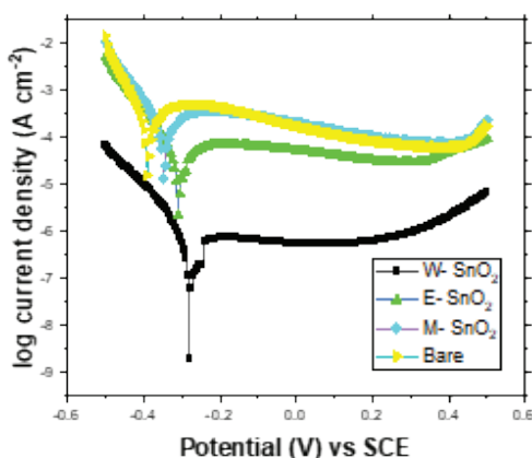
Fig. 5: Potentiodynamic polarization plots of the SnO 2 sample in sea water
