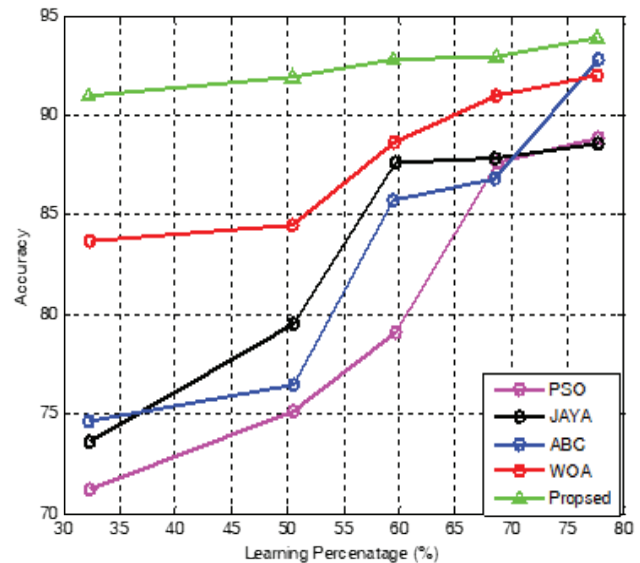
Fig. 4: Accuracy
