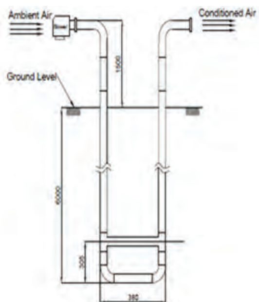
Fig. 8: Simulation of Vertical
