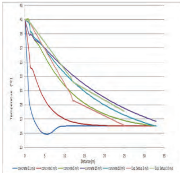
Fig. 9: Temperature of air travel in Horizontal BTHE at different air velocity
